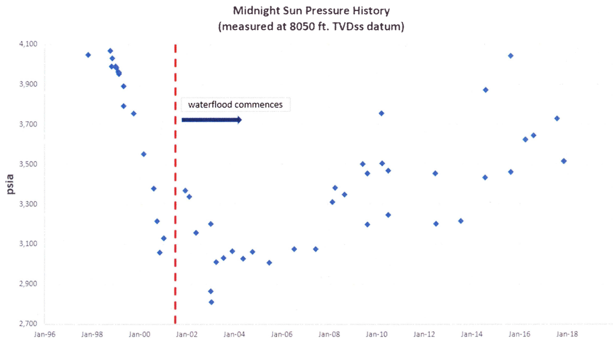
FIGURE 4: Midnight Sun Well Reservoir Pressure (measured at 8050 TVDSS Datum)
