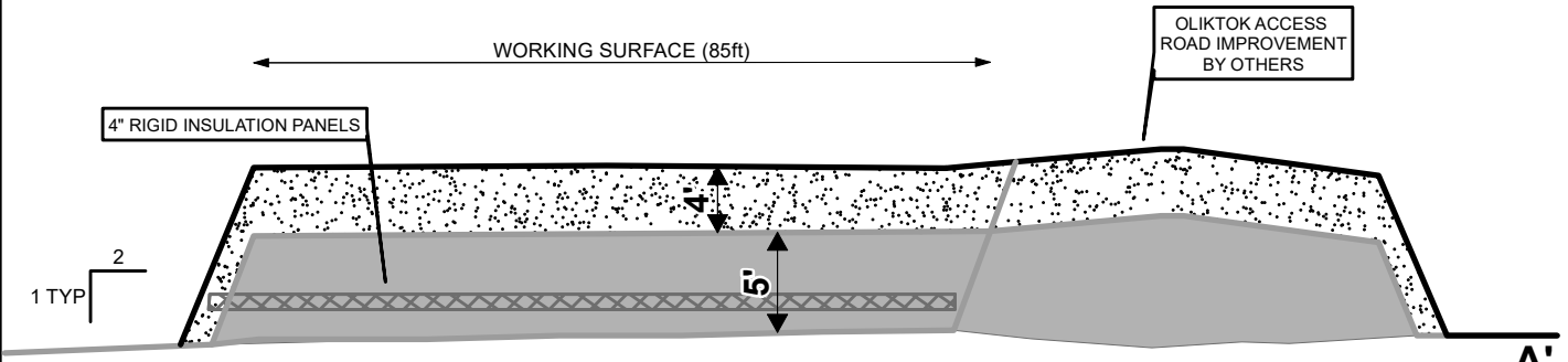
A 8' CROSS SECTION NOT TO SCALE
